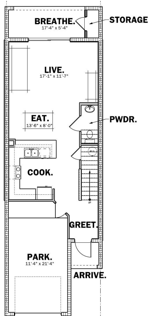
1st FLOOR PLAN UNIT "F" INTERIOR UNIT
