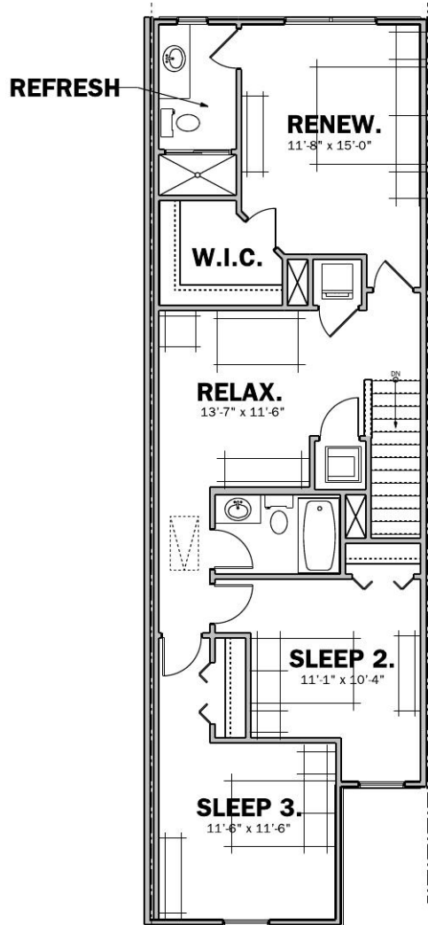
2nd FLOOR PLAN UNIT "F" INTERIOR UNIT
