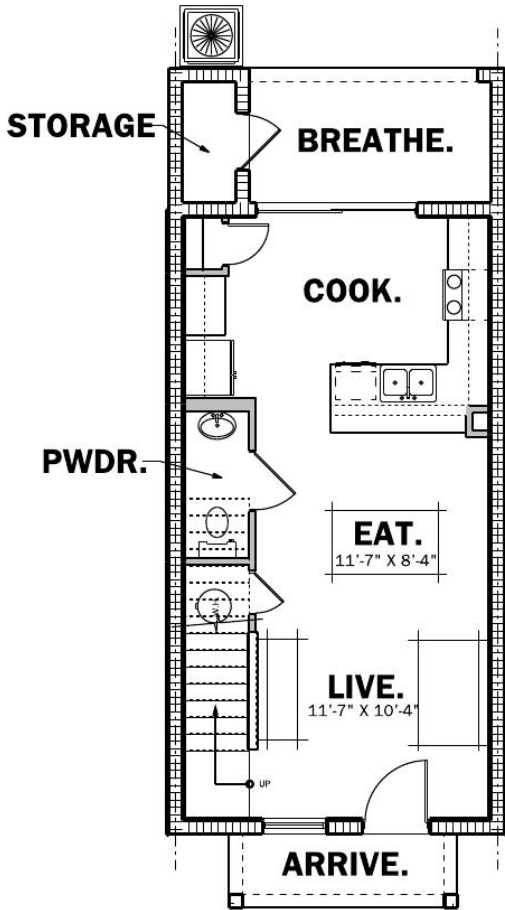
1st FLOOR PLAN UNIT "C" INTERIOR UNIT
