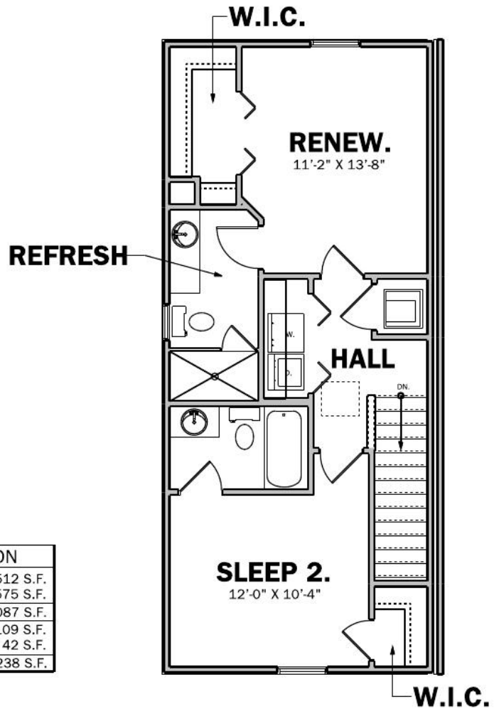
2nd FLOOR PLAN UNIT "B" EXTERIOR UNIT
