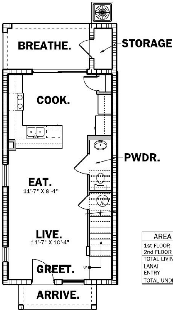
1st FLOOR PLAN UNIT "B" EXTERIOR UNIT
