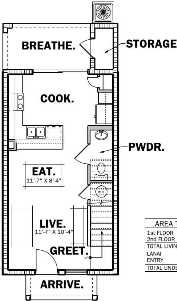
1st FLOOR PLAN UNIT "A" INTERIOR UNIT
